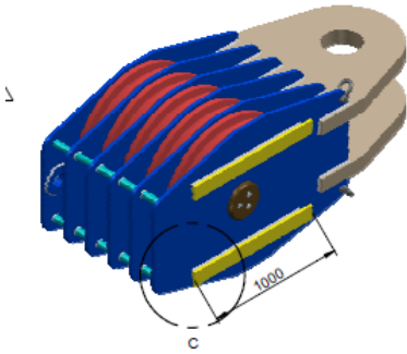
2 pcs Blocks WLL 500 tons 5 sheaves
