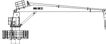
Item 5-11 Offshore Crane DNV Class unused Norsok SWL 5 ton and 13 mtr
